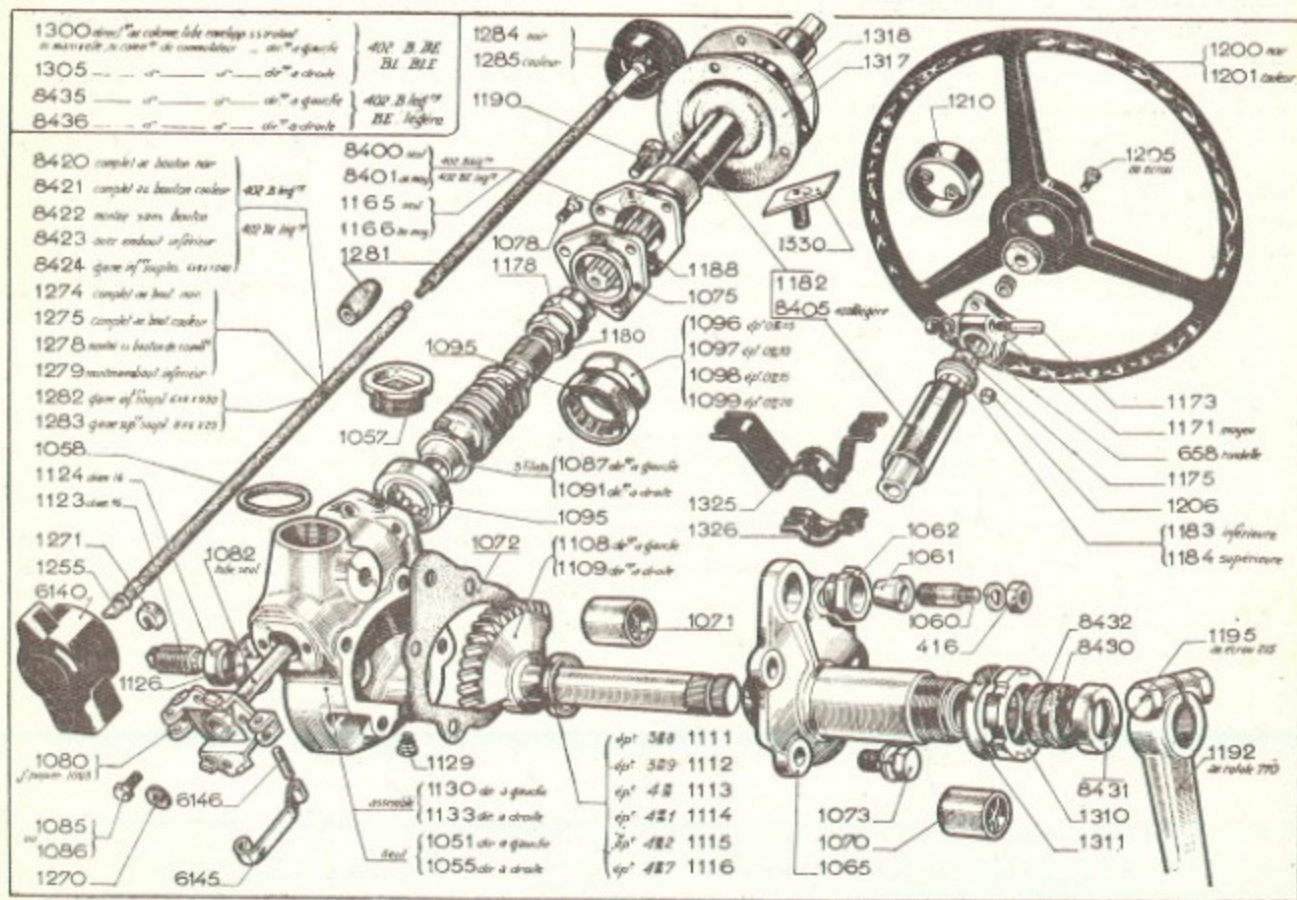
402 B. - Direction
