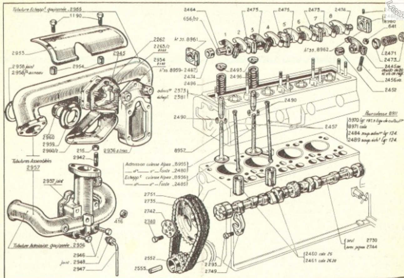
402 B. — Distribution
